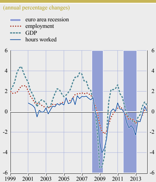
Chart 4 Employment, hours and GDP growth since 1999
