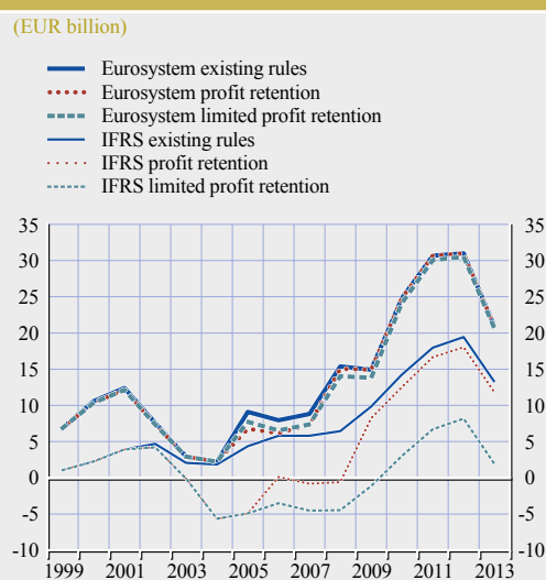
Chart 4 Simulation results for the financial buffers of the ECB (excluding capital)
