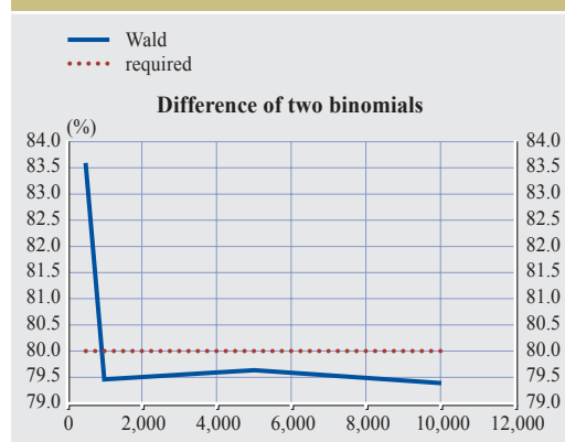
Chart 2 Performance of the Wald interval for differences of proportions
