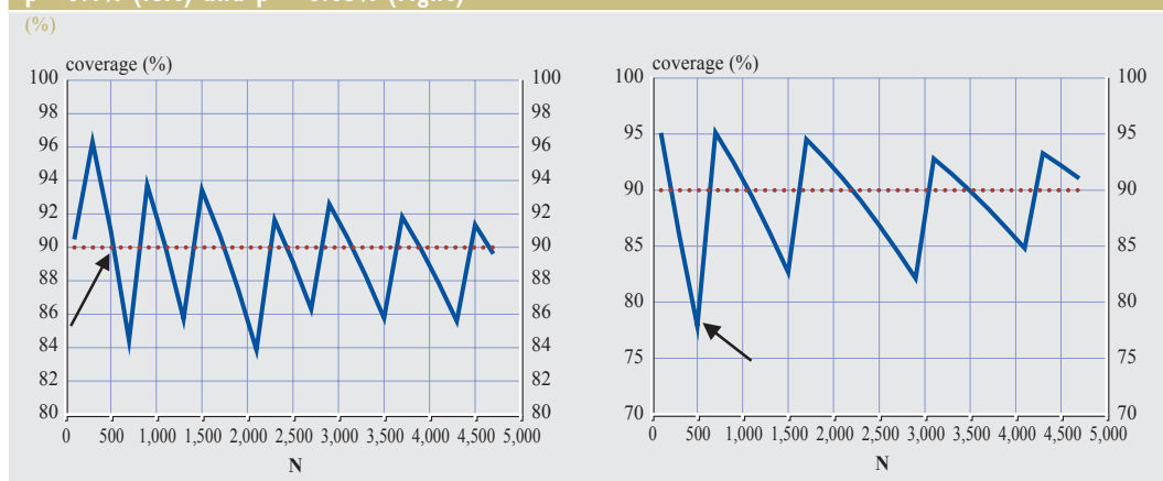
Chart 1 The performance of the Wald interval for different values of N , and for p = 0.1\% (left) and p = 0.05\% (right)
