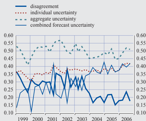
Chart 11 Short-term real unemployment rate forecast uncertainty
