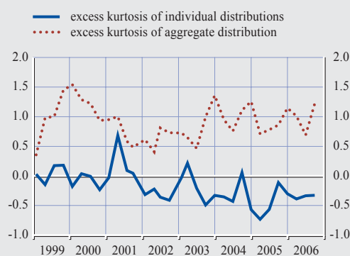
Chart 13 Kurtosis of short-term (one-year ahead) inflation forecasts
