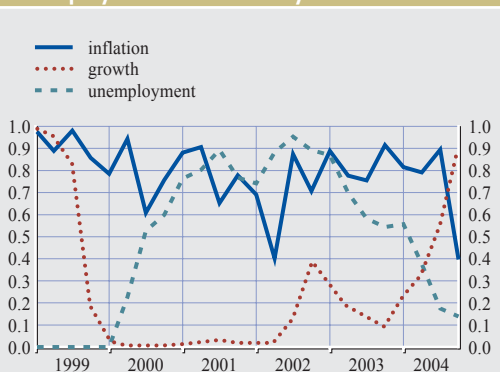
Chart 33 Probability integral transforms for two-year ahead inflation, GDP growth and unemployment rate density forecasts
