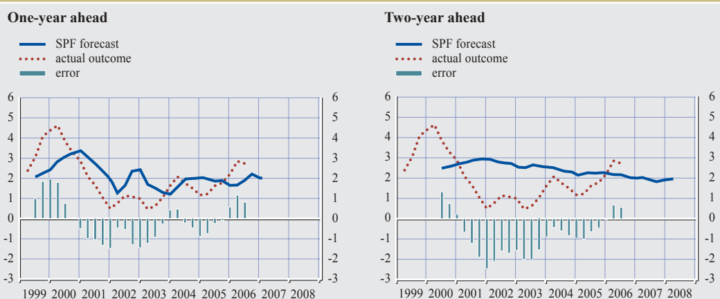
Chart 2 One and two-year ahead forecasts of real GDP growth
