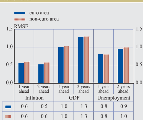
Chart 8 Average forecast errors (RMSE) for forecasters based inside and outside the euro area
