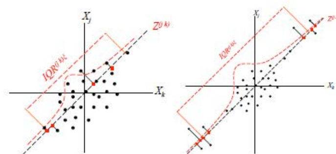
Figure 1. Source: Ricci and Veredas (2013) , Figure 1 at page 34. Diagrammatic representation of TailCor. Scatter plots, along with the 45-degree line, where X_j and X_k are positively related (the pairs are depicted with circles). Left plot shows a linear relation while right plot shows a nonlinear relation. Projecting the observations onto the 45-degree line produces the random variable Z^{(jk)} , depicted with squares. For illustrative purposes the projection is shown only for the observations on the tails but in the estimation it is done for all the observations.
