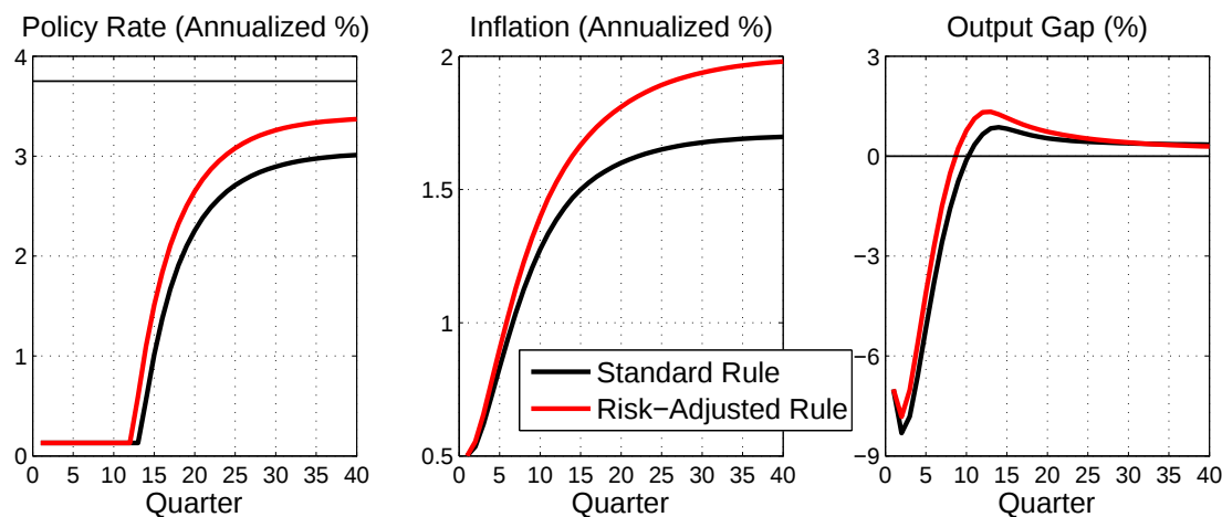
Figure 1: Modal Forecasts from a Model with ELB
