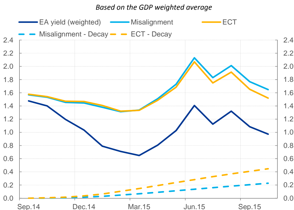
Figure 4: The dynamic impact of APP on 10-yr sovereign yields: A counterfactual analysis (percentage points)
