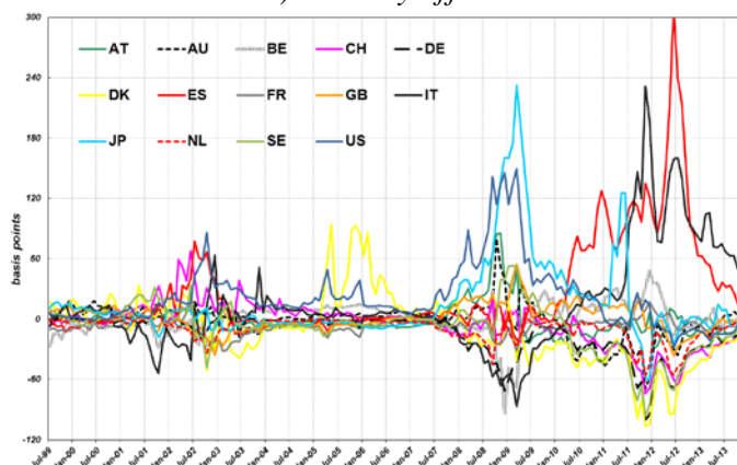
d) cross-sectional dispersions
