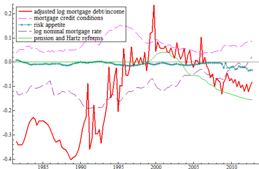
Figure 5.4a: Decomposition of adjusted long-run solution for log mortgage stock/income: mortgage credit conditions, risk appetite, the mortgage interest rate and pension and labour market reform.
