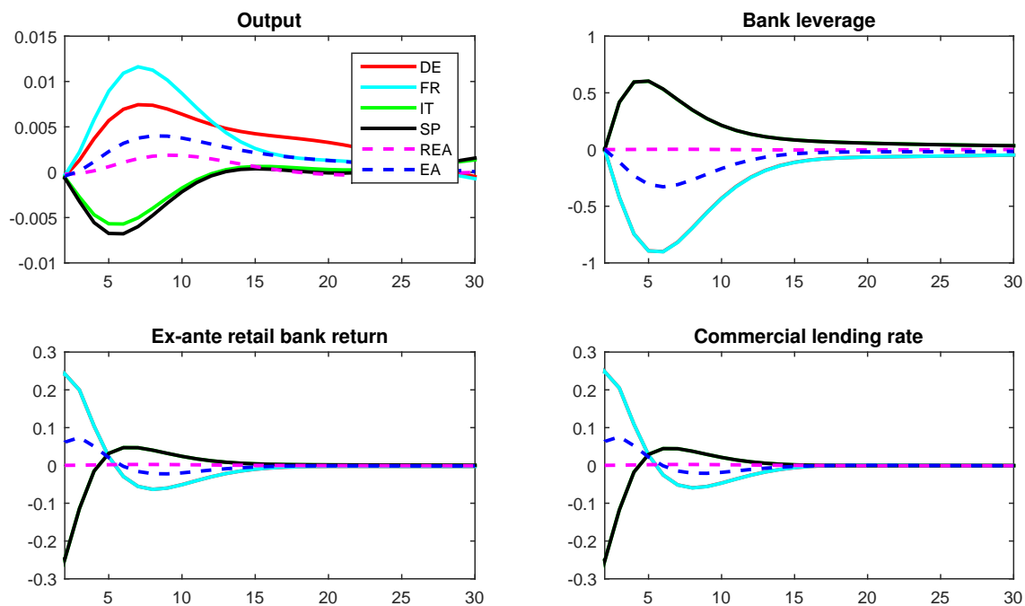
Figure 37: Increase euro area sovereign risk premium - Asymmetric staggered lending rate setting calibration (difference from symmetric case)
