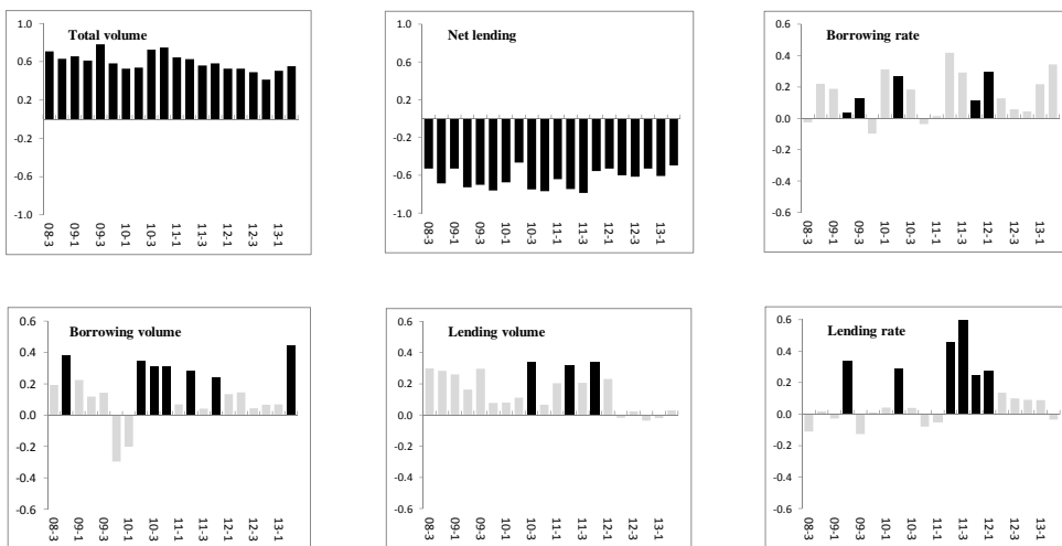
Figure 3: Estimates of Spatial Correlation Coefficients from Cohen-Cole equation
