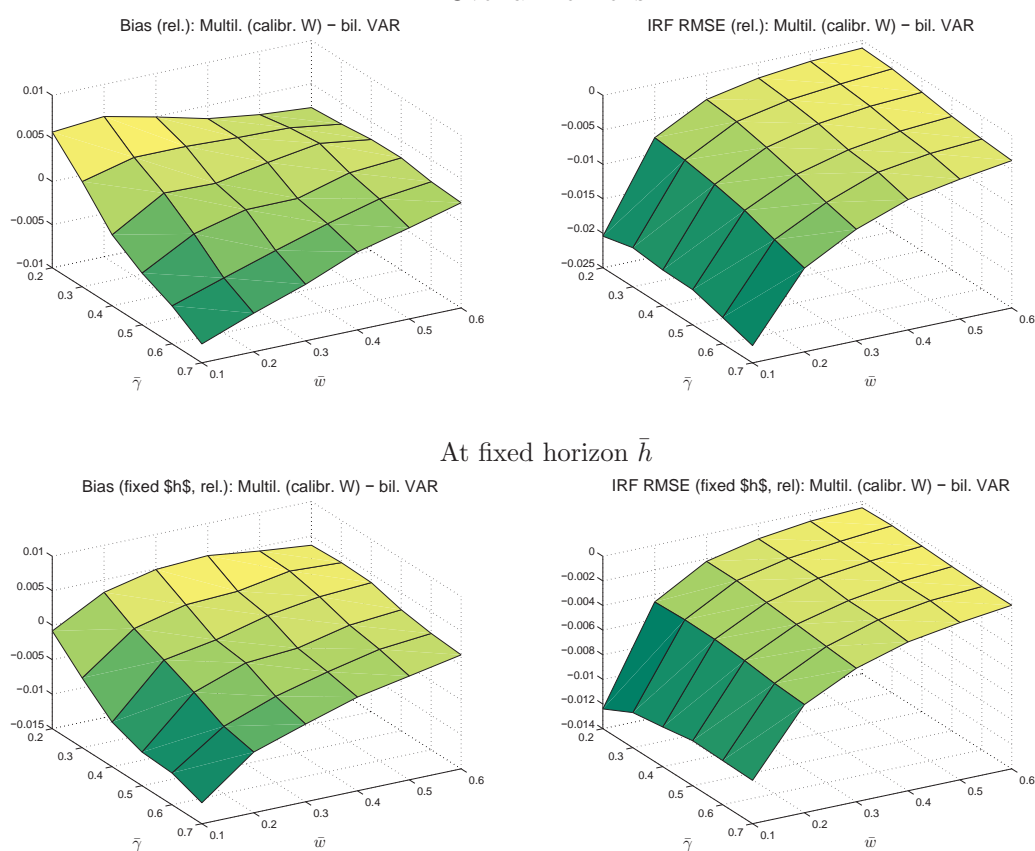
Figure 5: Difference Between Bias and RMSE of Spillover Estimates Obtained from the Multilateral with Calibrated Weight Matrix C and the Bilateral Model Over all horizons
