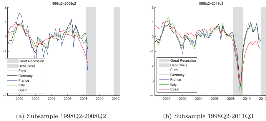
Figure 7: Estimated euro area and country factors using different subsamples: (a) subsample 1998Q2-2008Q2 and (b) subsample 1998Q2-2011Q3
