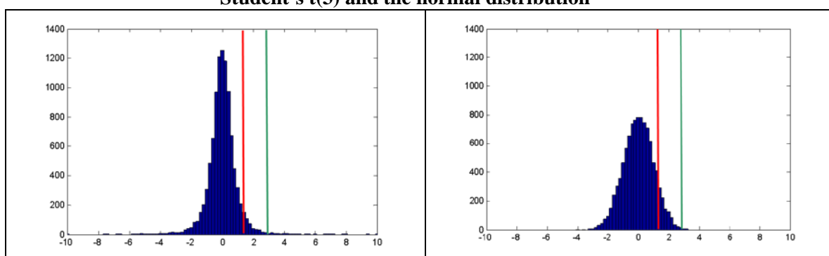
Chart B1. Comparison of histograms with 1.5 and 3 standard deviation thresholds of Student's t(3) and the normal distribution
