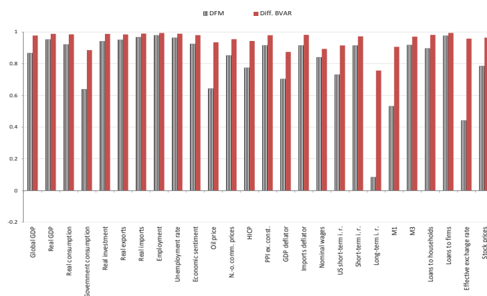
Figure 1: Correlation of DFM and BVAR in differences forecasts with BVAR in levels forecasts (a) One quarter ahead
