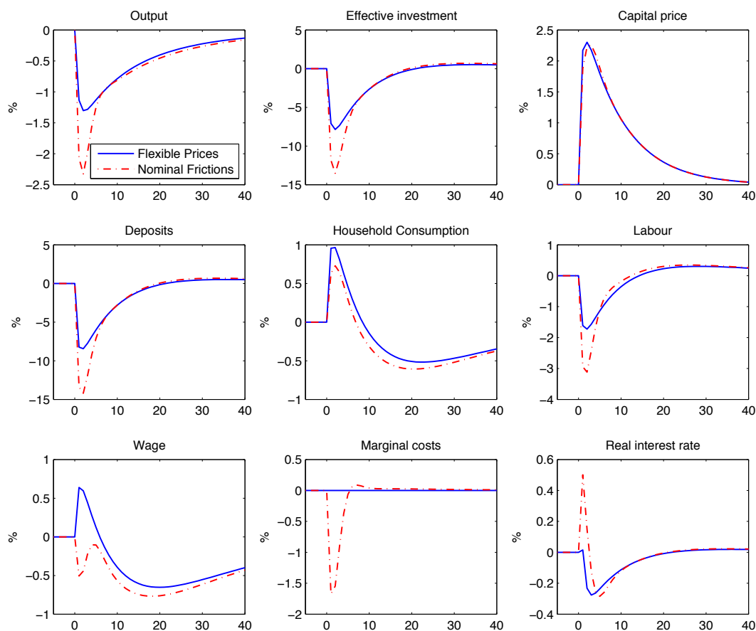
Figure 5: Responses to a Collateral Shock with Nominal Frictions
