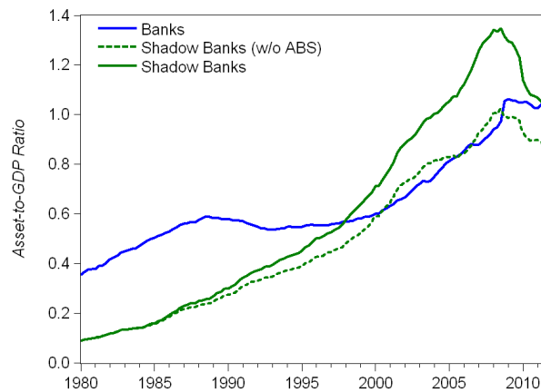
Figure 7: Asset-to-GDP Ratios of Banks and Market-based Intermediaries
