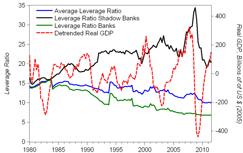
Figure 6: Leverage Ratios of Banks and Market-based Intermediaries
