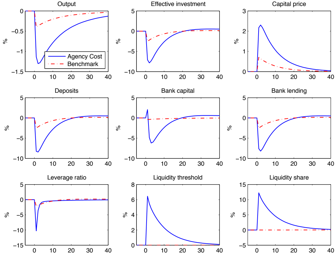
Figure 4: Responses to a Collateral Shock
