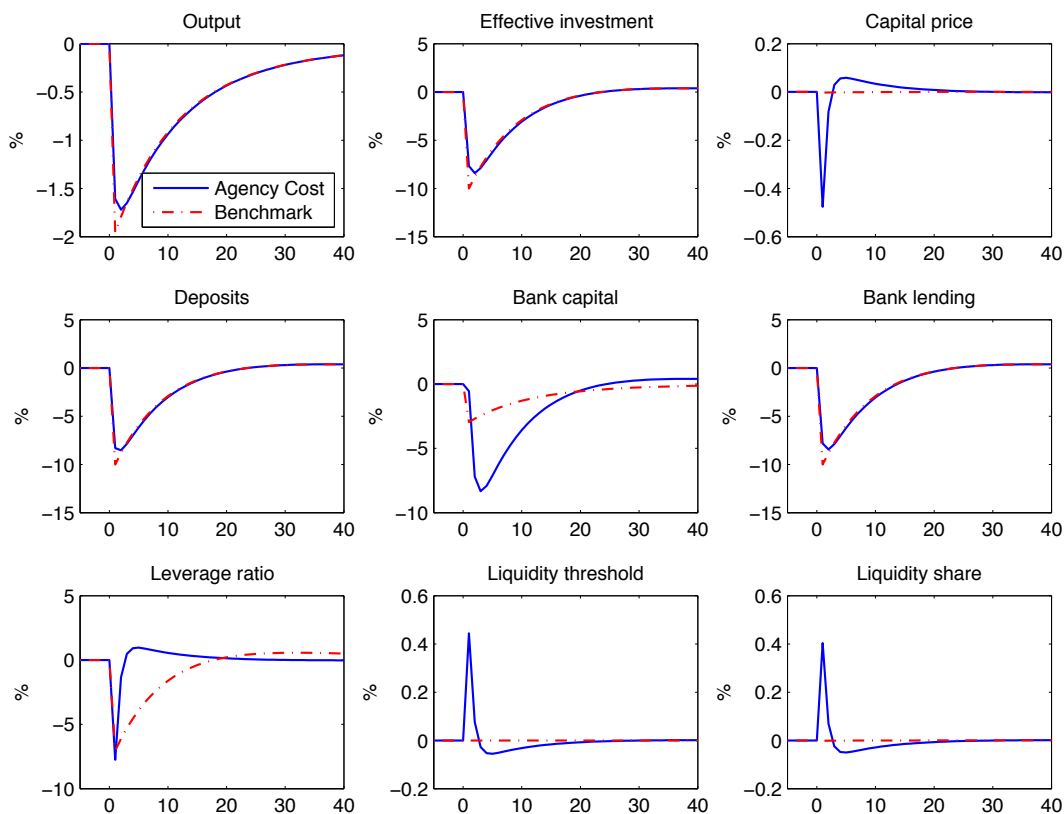
Figure 3: Responses to a Technology Shock
