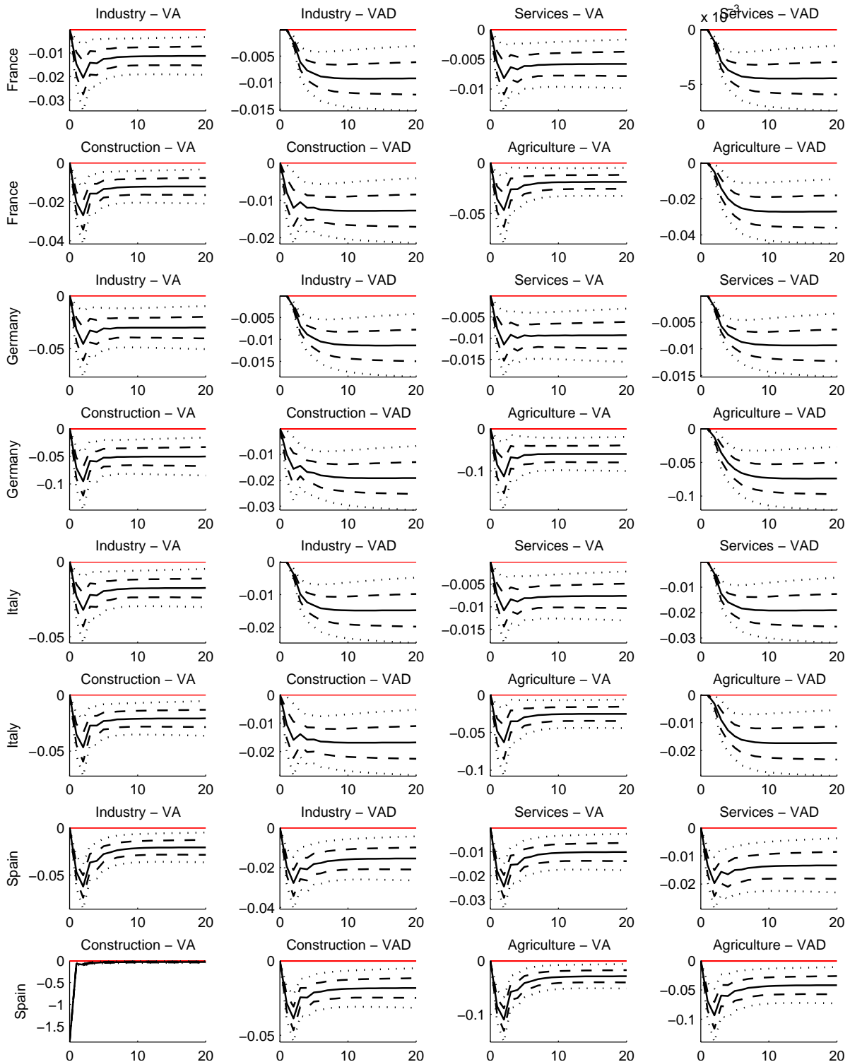
Figure 10: Impulse response functions of selected variables to a one-standard-deviation shock to total real VA in Spanish construction based on the multi-country PVAR model (Point estimates with one and two-standard error confidence intervals)
