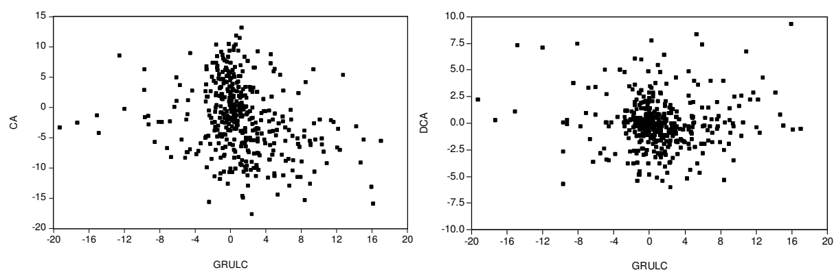
Figure 1: Crossplots GRULC and CA or DCA; annual data 1997–2012, 27 EU countries
