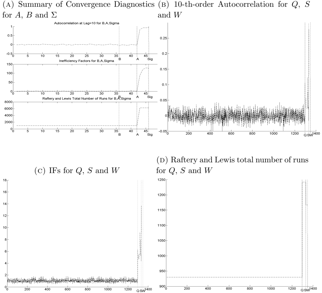
FIGURE 12. Convergence Diagnostics
