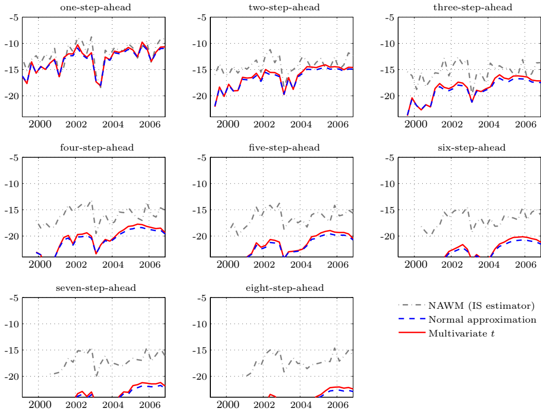
FIGURE 12: Log predictive likelihoods for the large selection of variables using the random walk model.
