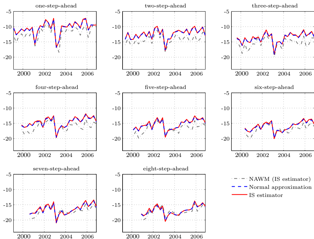
FIGURE 10: Log predictive likelihoods for the large selection of variables using the DSGE-VAR(2) model.
