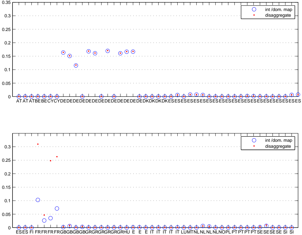
Figure 7: SPI index for two different Probability Maps (for grouped banks into domestic/internationally active banks and for disaggregate data)
