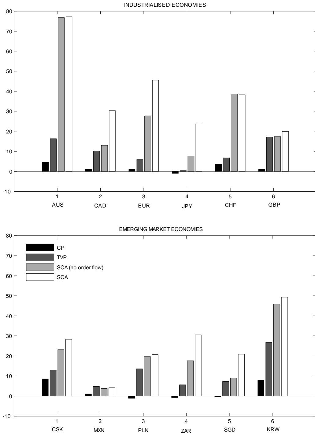
Figure 2 Unconditional adjusted- R^2
