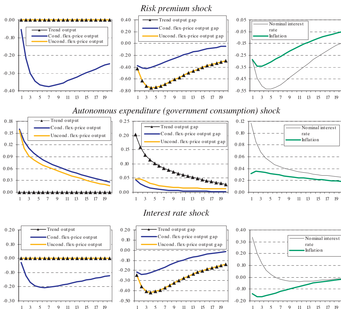
Figure 1.2. Impact of demand and monetary shocks
