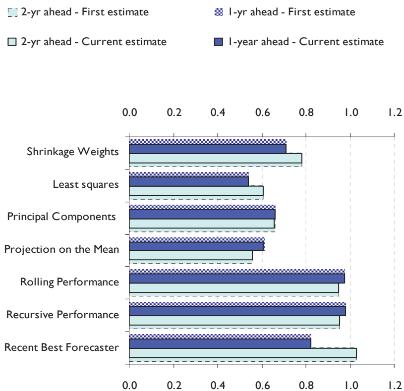
(b) Inflation
