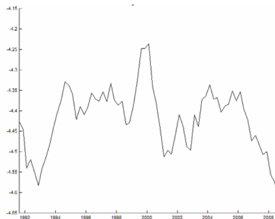
Cointegration relationship
