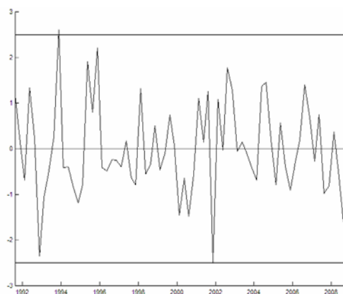
Normalised residuals
