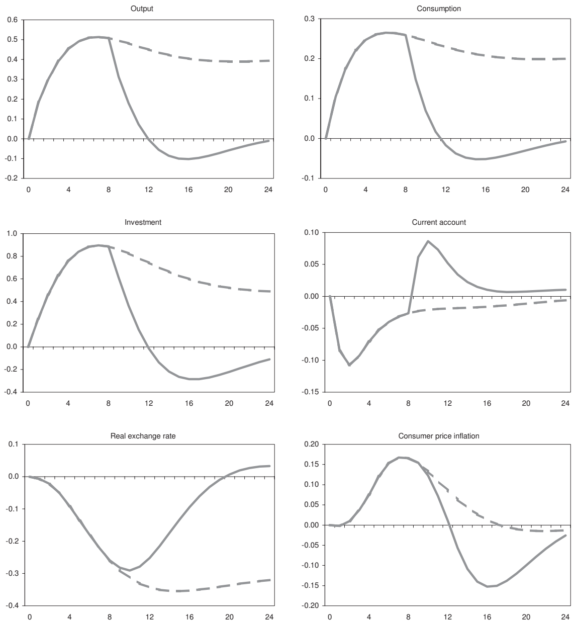
Figure 4. Transitory (but perceived as permanent) productivity shock in the tradable sector
