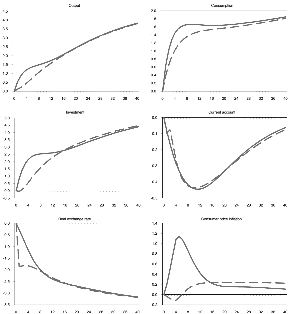
Figure 6. Dynamic responses to productivity convergence in the tradable sector: different regimes
