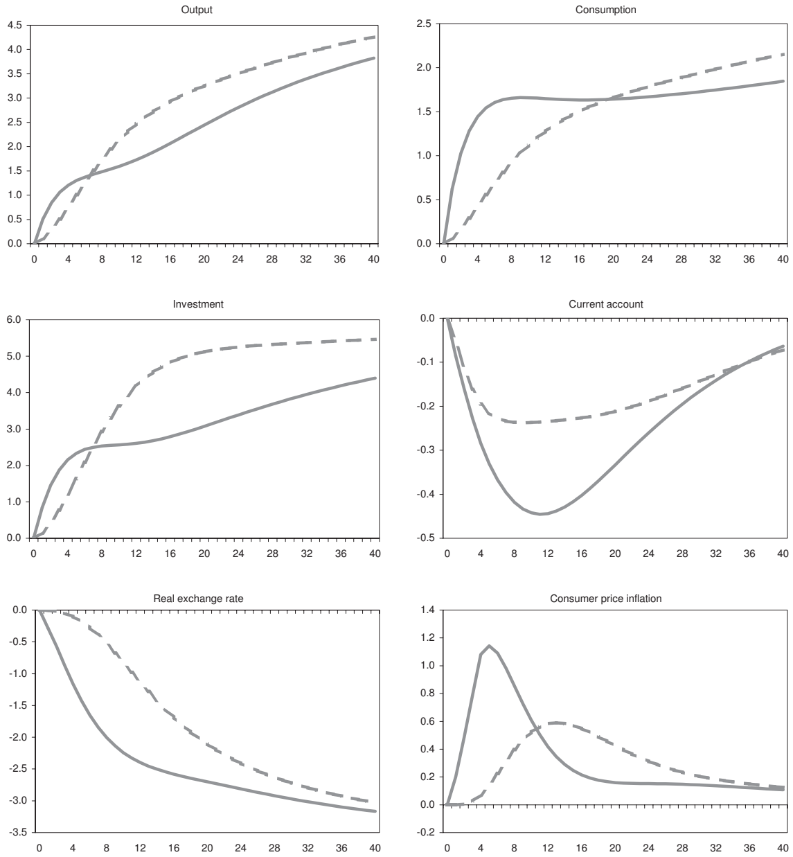
Figure 2. Dynamic responses to productivity convergence in the tradable sector
