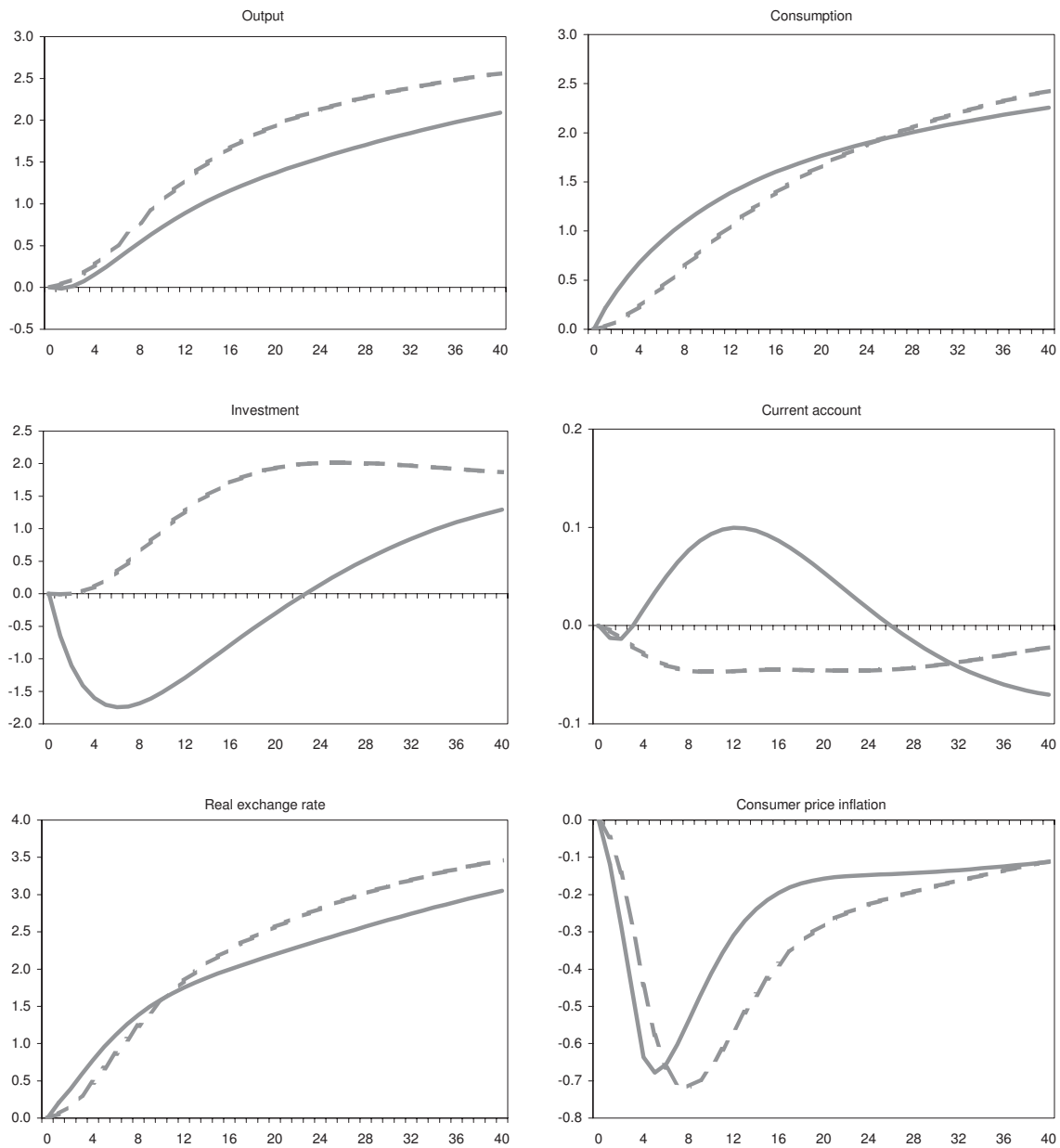
Figure 3. Dynamic responses to productivity convergence in the nontradable sector
