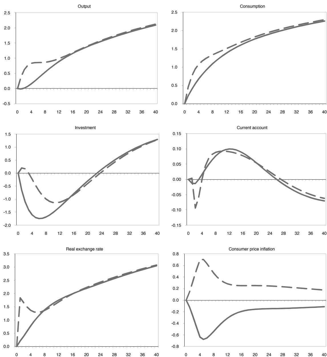
Figure 7. Dynamic responses to productivity convergence in the nontradable sector: different regimes
