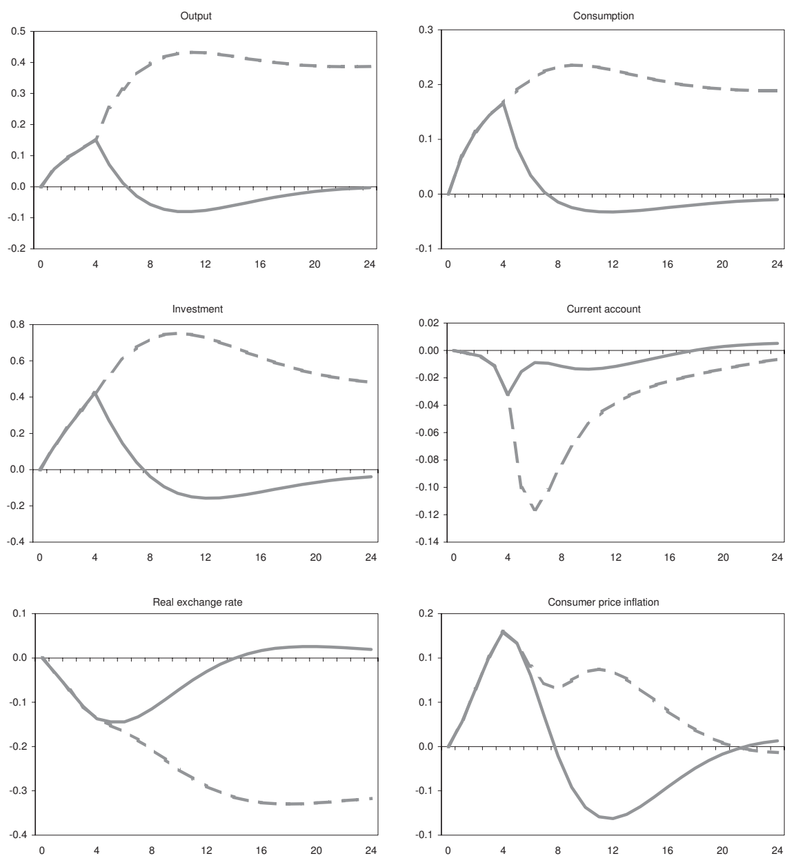
Figure 5. Expected (but failing to materialize) productivity shock in the tradable sector
