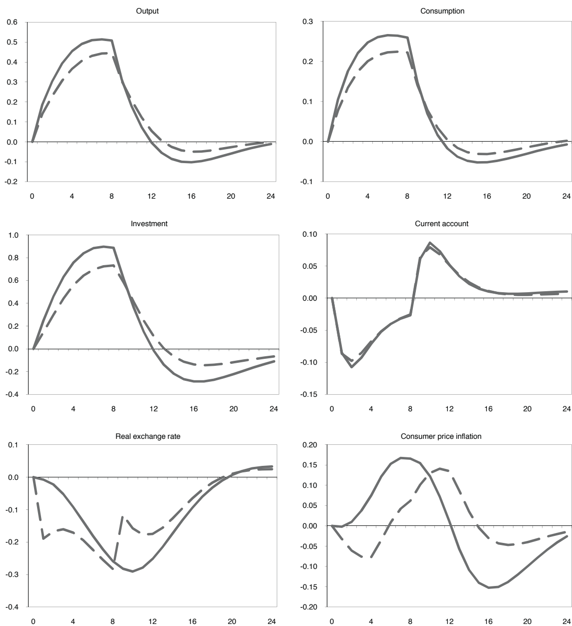
Figure 8. Transitory (but perceived as permanent) productivity shock in the tradable sector: different regimes
