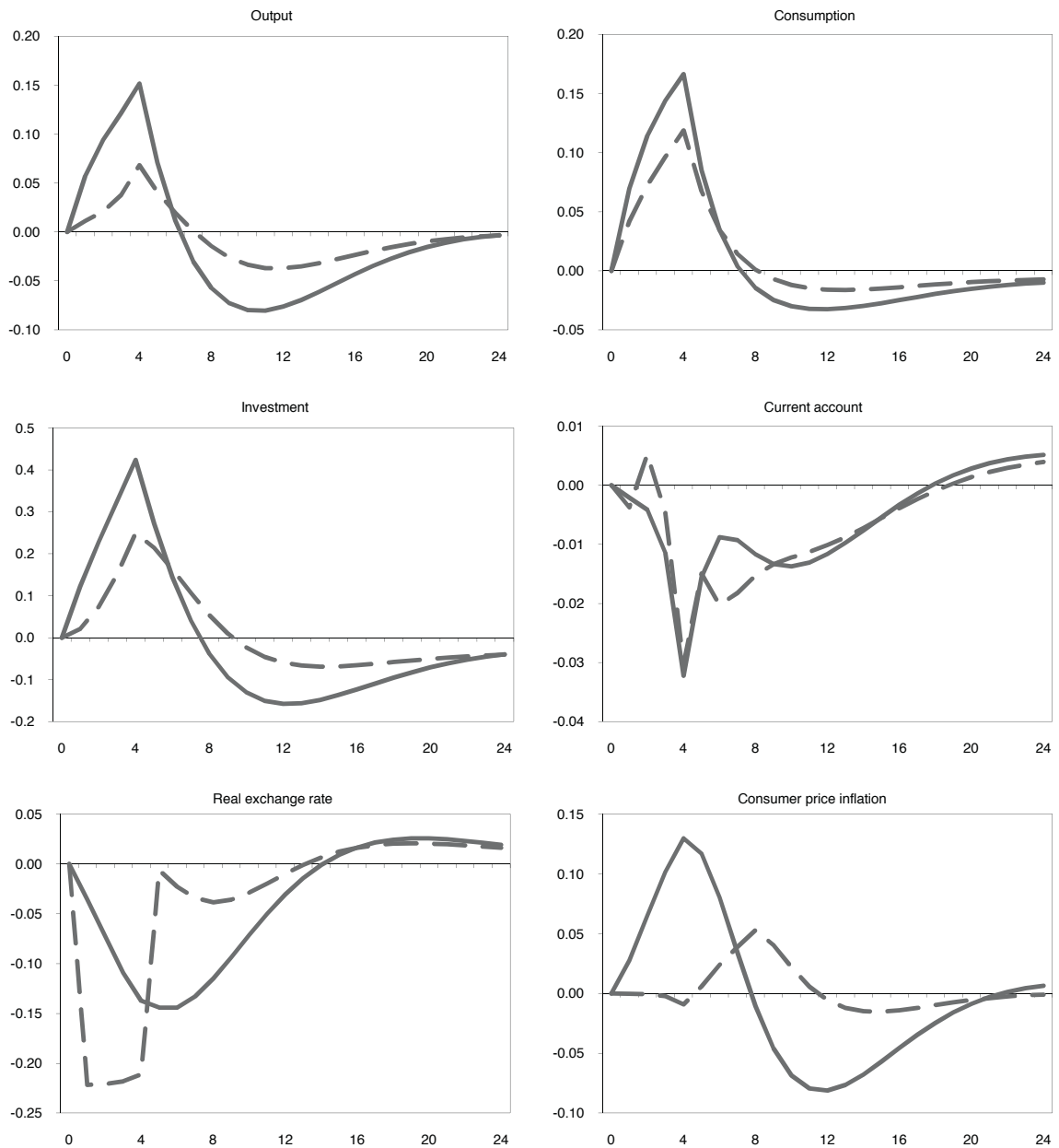
Figure 9. Expected (but failing to materialize) productivity shock in the tradable sector: different regimes
