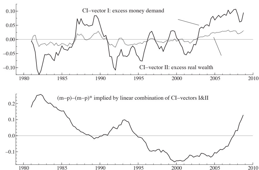
Figure 26: Measures for "excess money "
