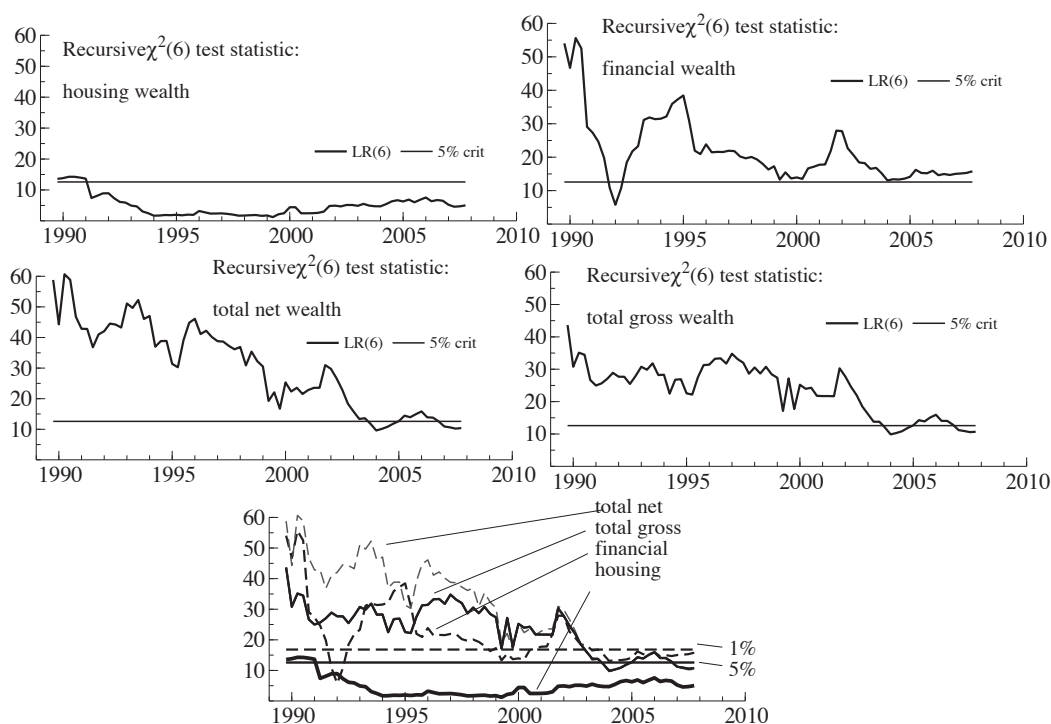
Figure 7: Alternative wealth aggregates: recursive tests for the validity of identification scheme
