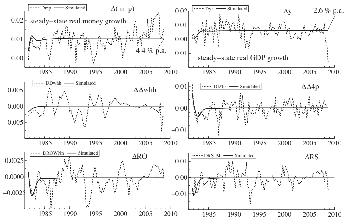
Figure 20: VECM: actual and simulated long-run steady state values
