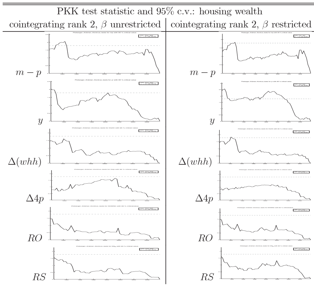
Figure 15: Ploberger-Krämer-Kontrus test statistics
