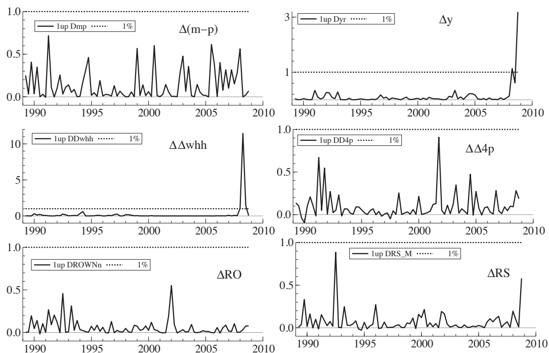
Figure 22: 1-step ahead "Chow" tests for individual equations of the VECM
