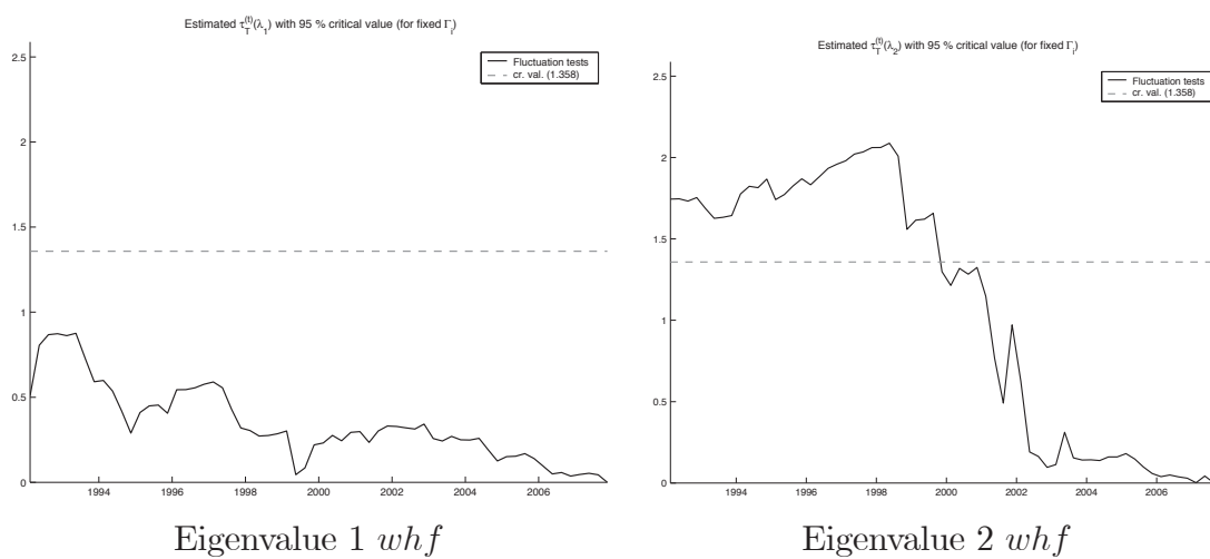
Figure 11: Fluctuation test whf
