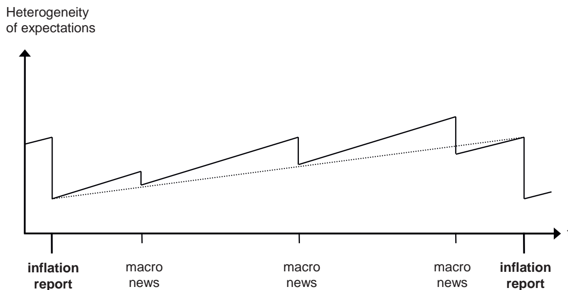
Figure 2: The predicted evolution of expectation heterogeneity
