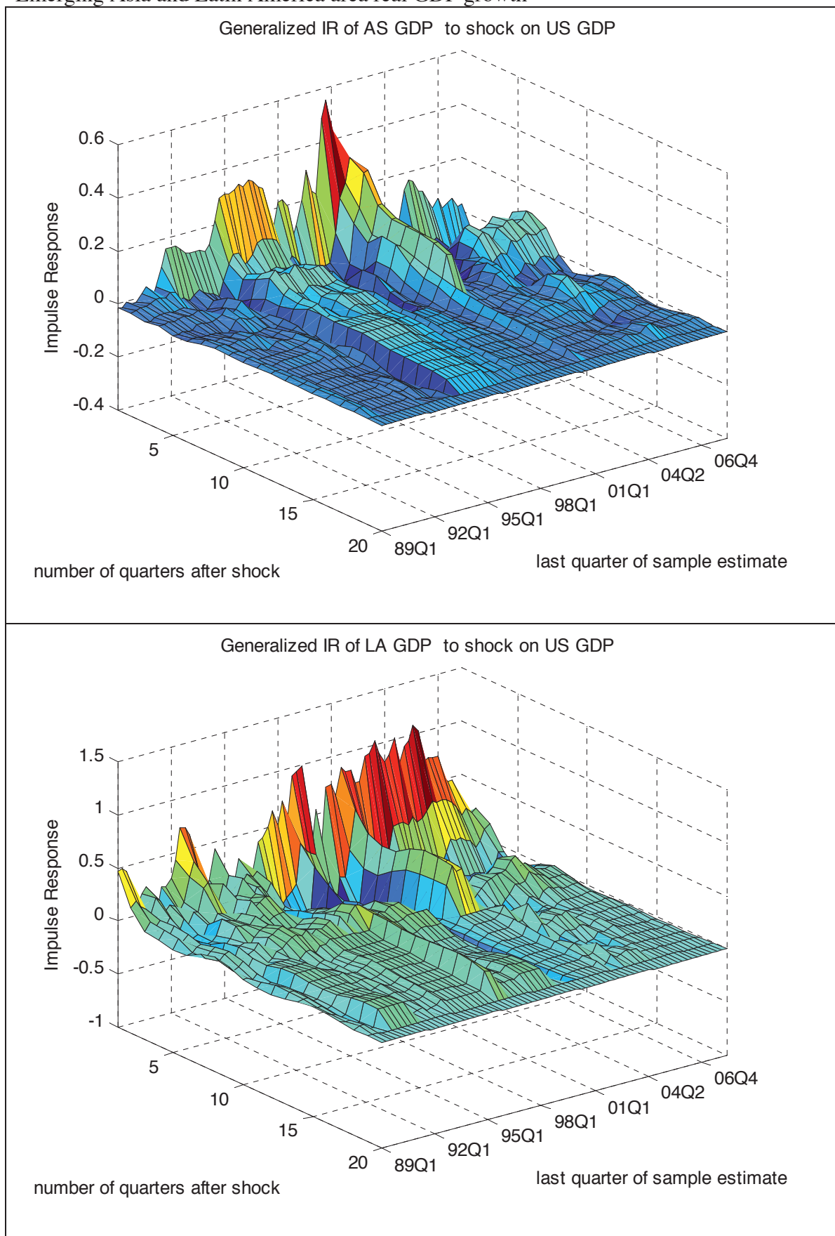
Figure 5 (cont'd) - Impulse response functions of a 1% shock to US real GDP on Emerging Asia and Latin America area real GDP growth
