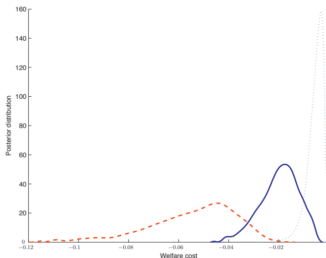
Figure 2: Welfare costs of the estimated rule and the optimized rule on the Volker-Greenspan sample .
