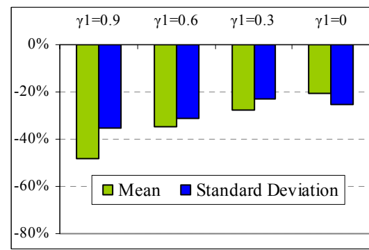
Figure 5: Overall gains from LS,N (MAE)
