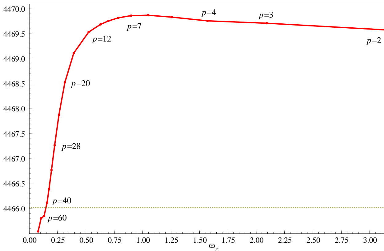
Figure 6: Profile likelihood for cut-off parameter \omega_c . The value p = 2\pi/\omega_c is the corresponding period in quarters.
