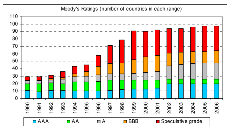
Figure 1 – Number of countries rated and rating categories
