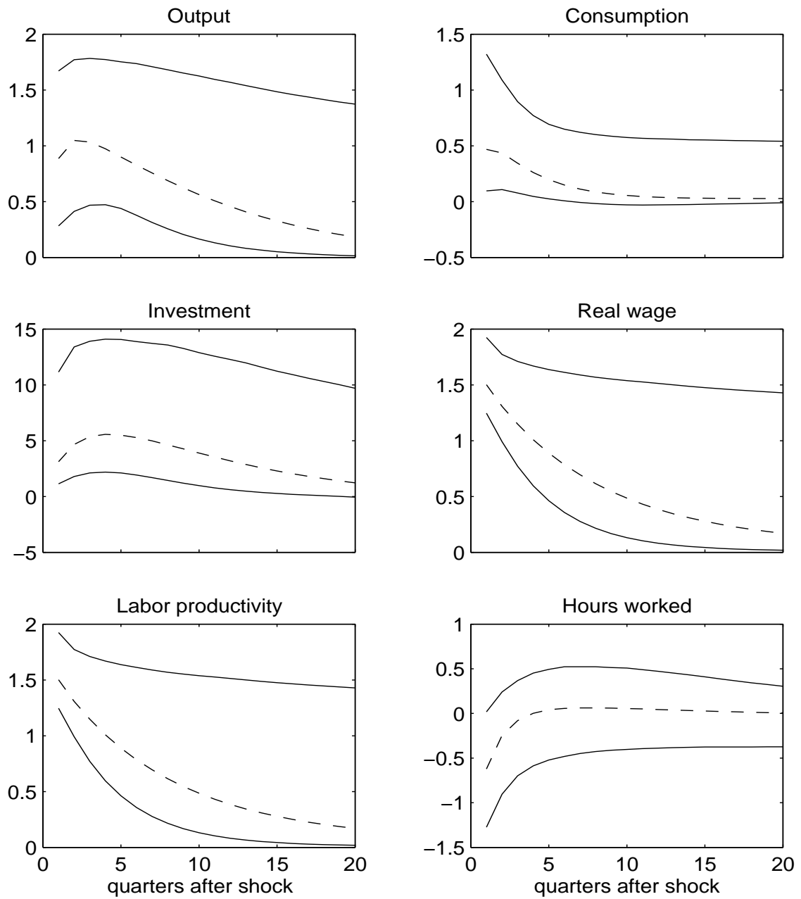
Fig. 1A Impulse responses to positive technology shock: RBC model
