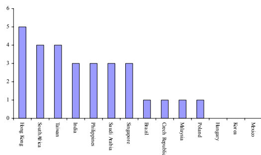
Figure 3: \Theta_i^*
