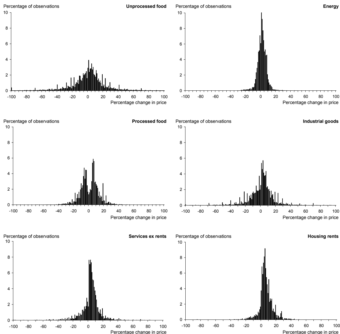
Figure 2: The distribution of price changes by components
