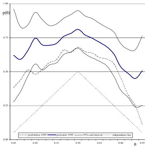
Figure 16i: Italy-Spain
