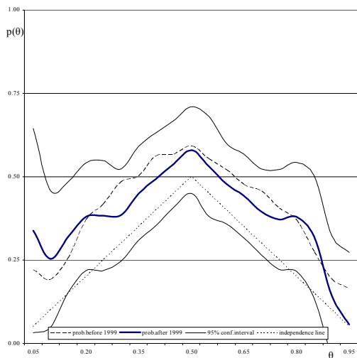
Figure 17g: Belgium-Greece
