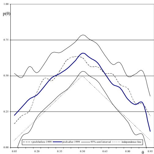
Figure 17i: Belgium-Portugal
