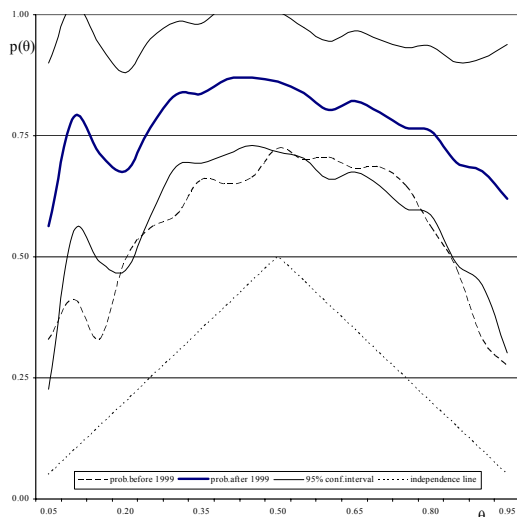
Figure 16c: France-Netherlands
