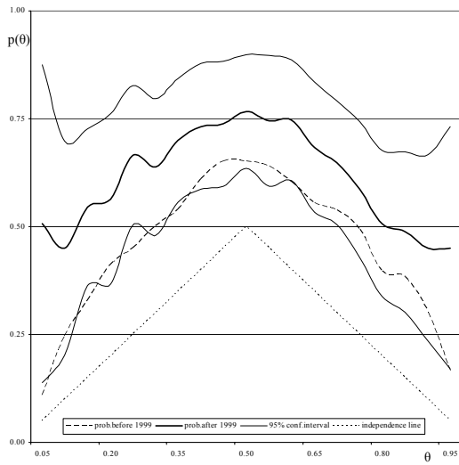
Figure 19g: US-UK
