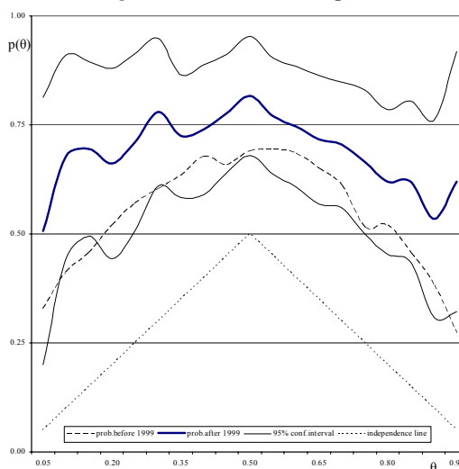
Figure 16d: France-Spain
