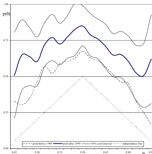
Figure 16d: France-Spain
