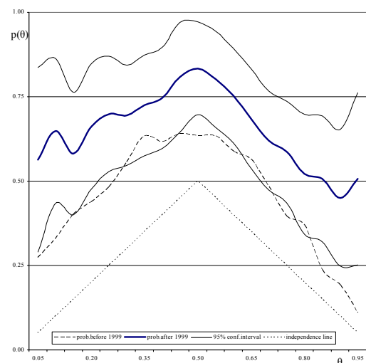
Figure 16j: Spain-Netherlands
