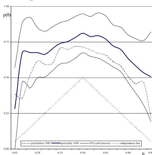
Figure 19d: Euro area-Sweden
