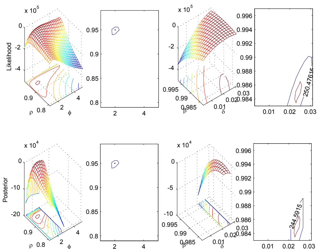
Figure 2: Likelihood and Posterior Surfaces and Contours
