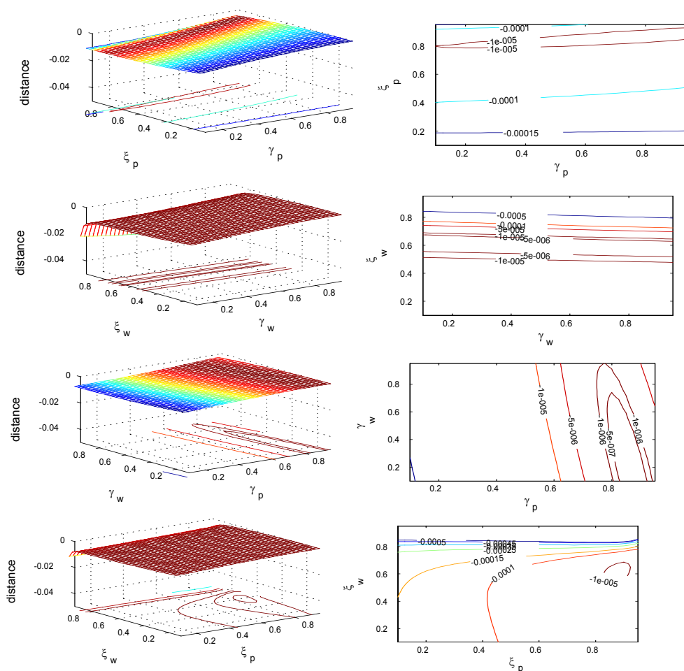
Figure 10: Distance surfaces and Contour Plots
