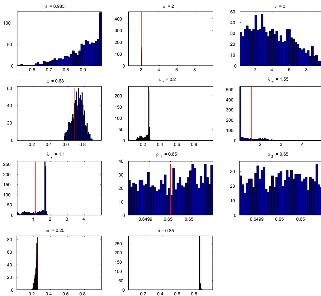
Figure 7: Distribution of estimates
