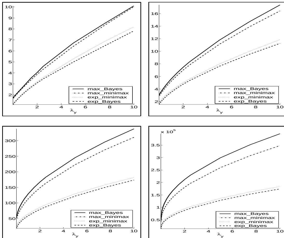
Figure 7: Minimax Losses vs. Bayesian Losses
