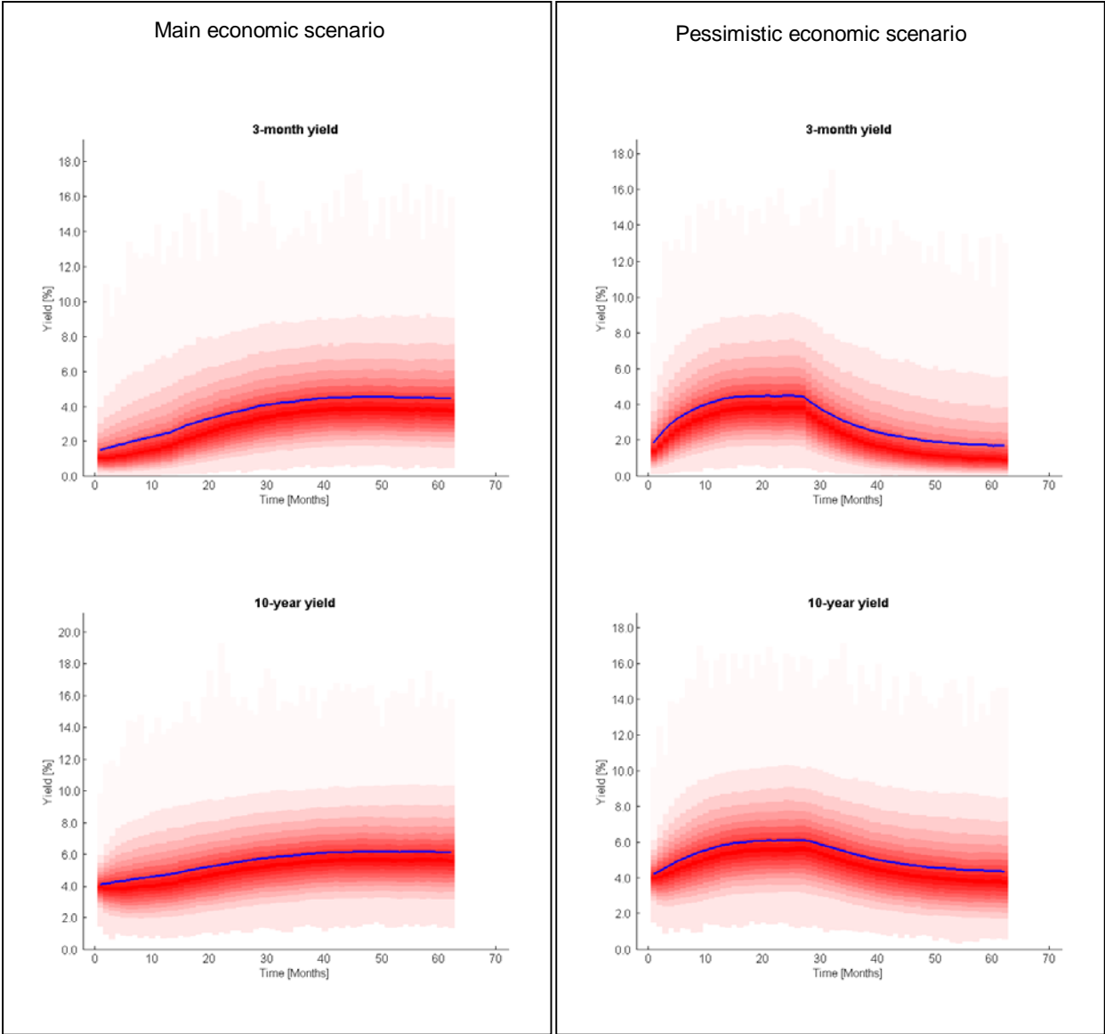
Figure 6: Distribution of 3 months and 10 years yields
