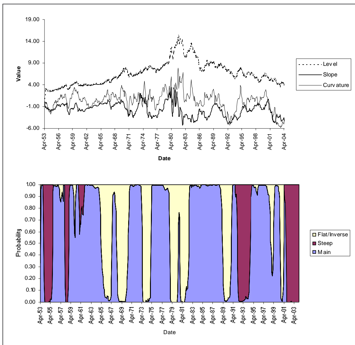
Figure 2: Estimates yield curve factors, regime classifications and generic yield curves
