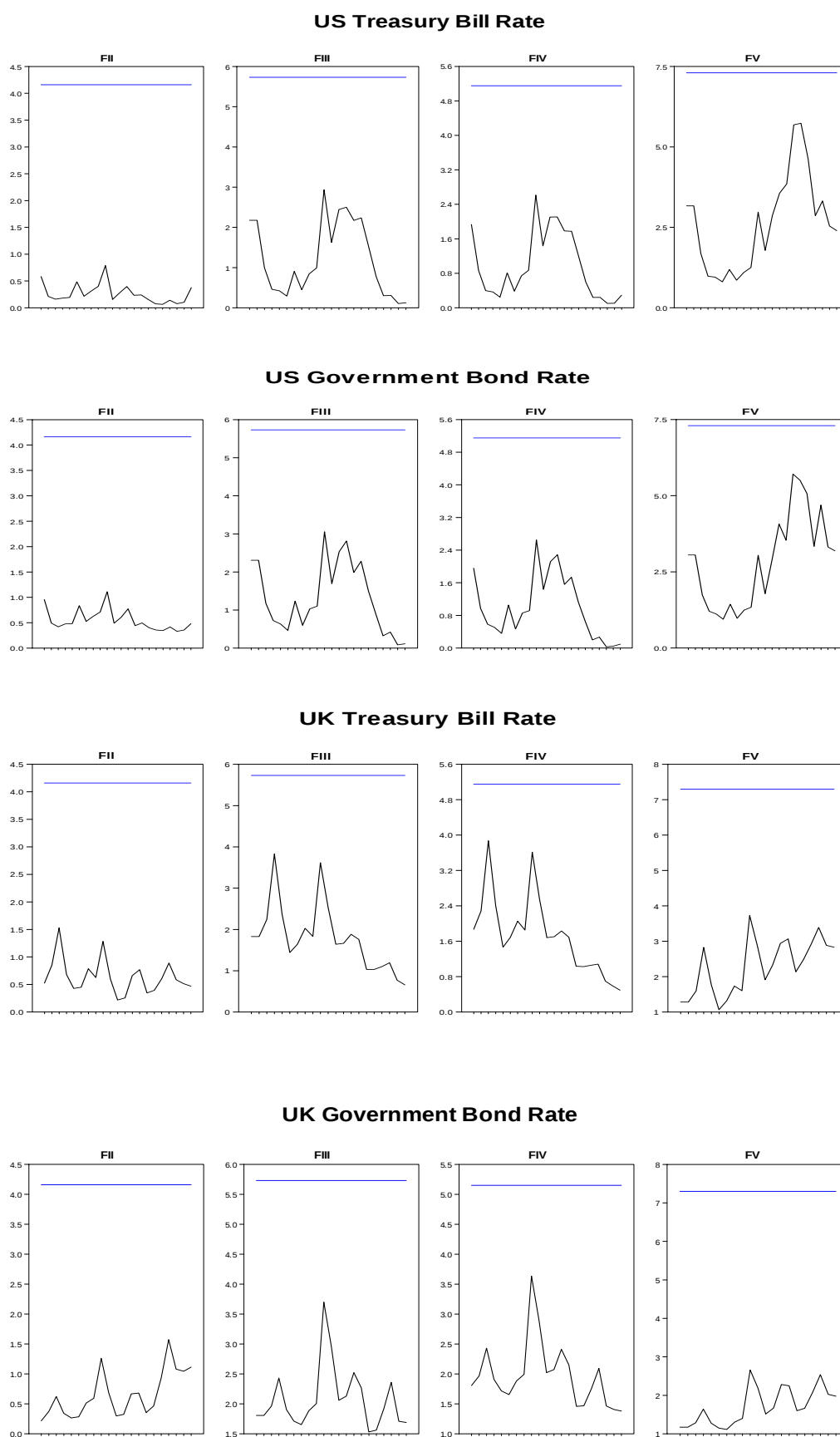
Figure 7: Bounds tests results: recursive estimates and fixed end point
