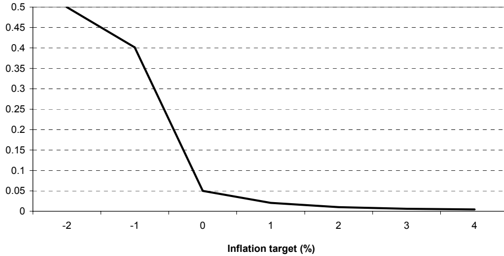
Figure 7: Probability of hitting the zero bound
