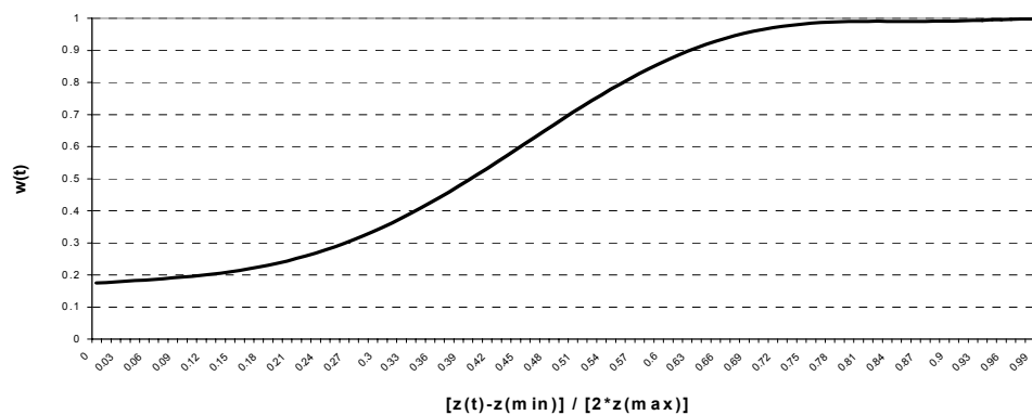
Figure 5: Weighting function ( \pi=-2\% )
