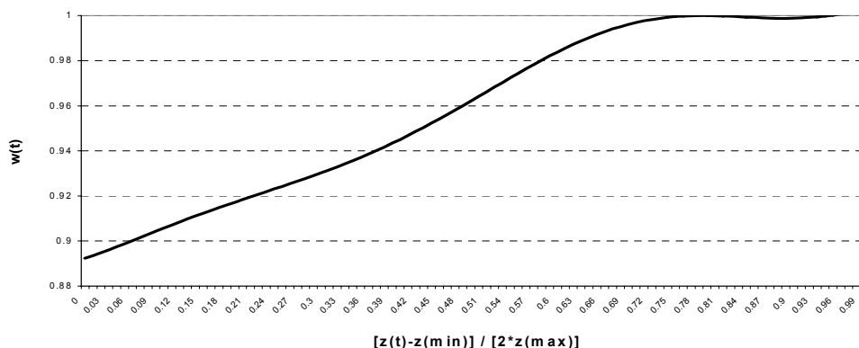
Figure 6: Weighting function ( \pi=2\% )
