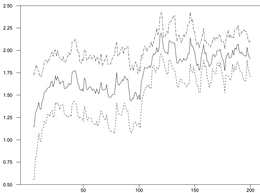
Figure 1. Posterior Distribution of \beta_t (Without Correction)
