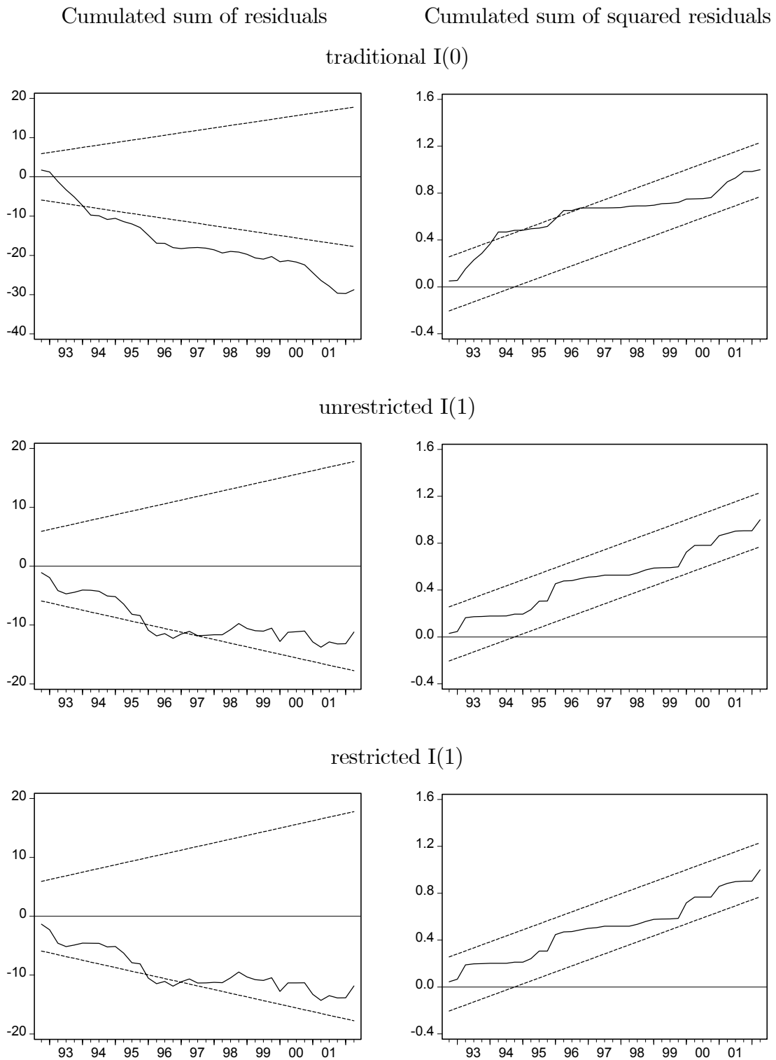
Figure 2: Cusum tests
