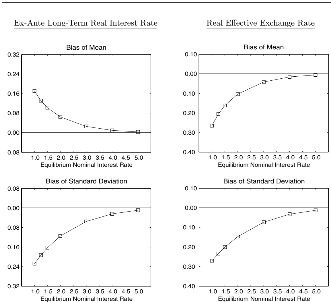
Figure 5: Distortion of Stationary Distributions of the Determinants of Output
