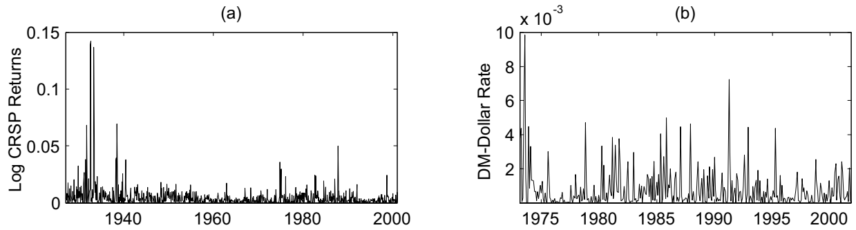
Figure 5.1: Squared Returns
