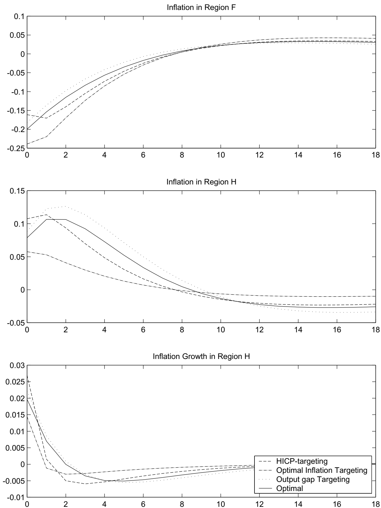
Figure 4: Impulse Response Functions, \alpha_H=0.75 , \omega_H=0.48 , \alpha_F=0.785
