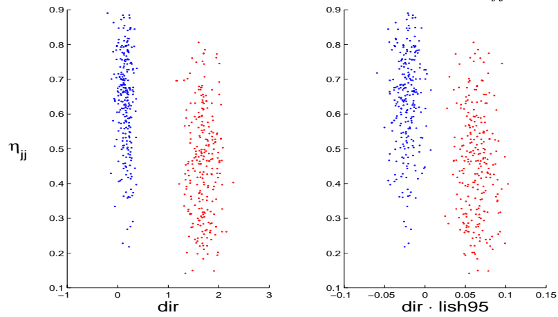
Figure 4: Scatter plot of simulated values for the coefficient on the interest rate ( \text{dir} ) and its interaction with liquidity ( \text{dir} \cdot \text{lish95} ) against persistence \eta_{jj} , respectively.
