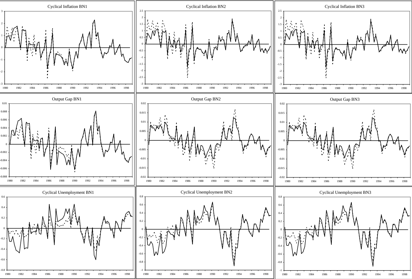
Final (solid line) vs Recursive (dashed line) Cycle Estimates. Euro Area – BN Models
