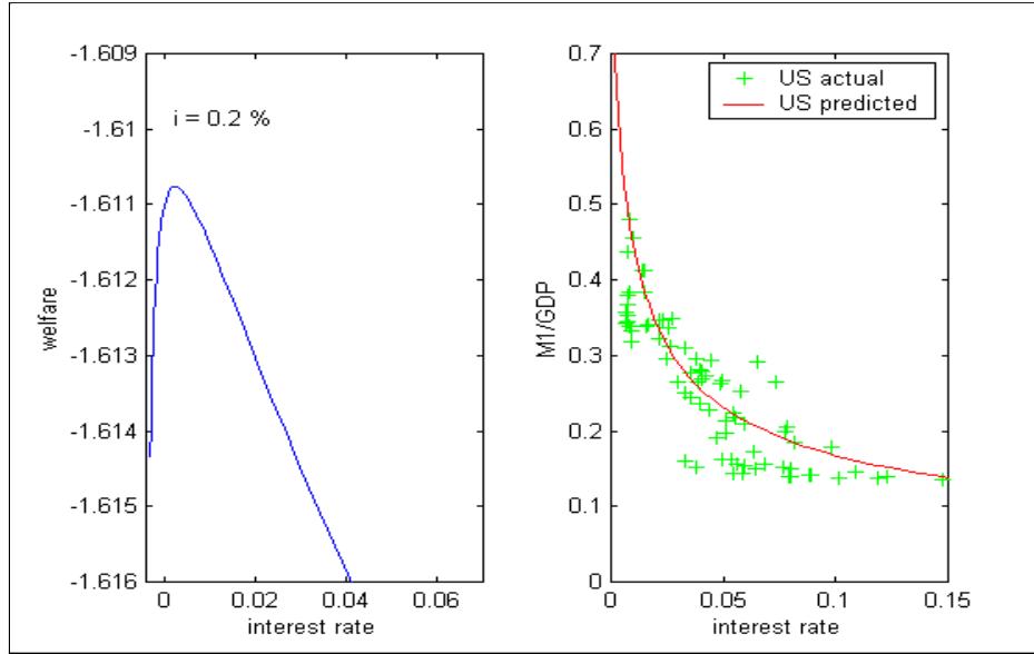
Figure 3: Benchmark case with \gamma = 1.05 , \frac{z}{g} = .1 , \frac{\bar{m}}{c} = 1 , k = 1 , \eta = .006 , \sigma = 1.8 , v = 1.3 .
